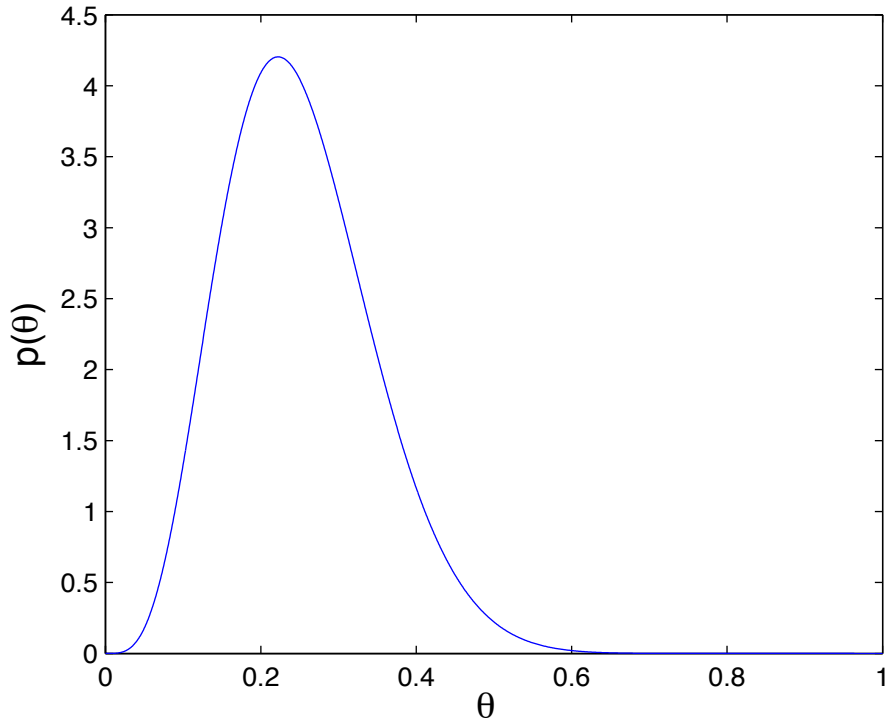
Prior distribution Beta(5,15)
