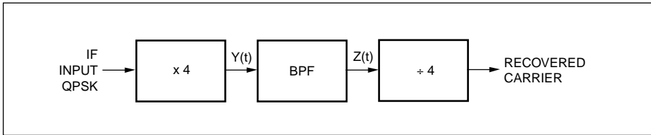
Figure 10. Multiply-filter-divide method of carrier recovery.
