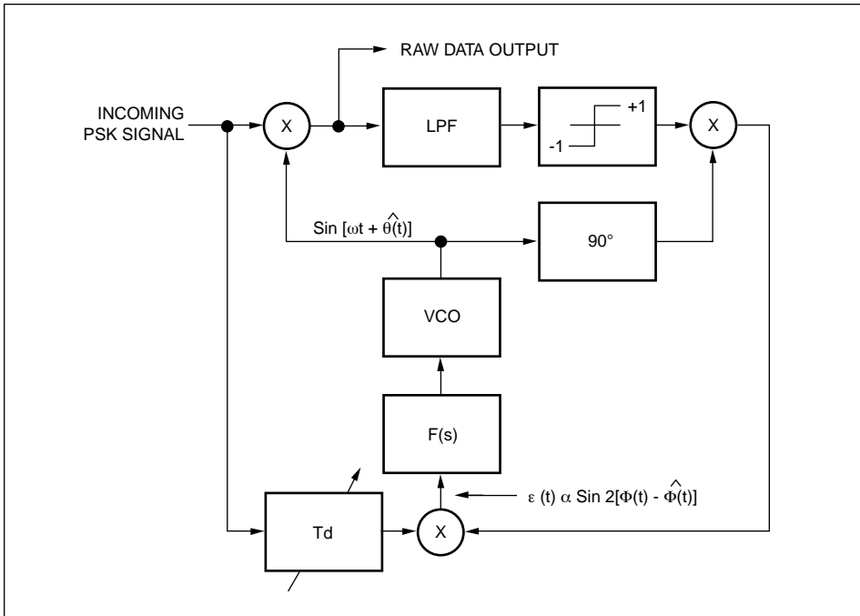
Figure 8. BPSK remodulator loop.
