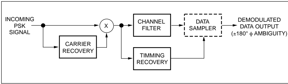
Figure 4. Block diagram of a PSK demodulator.
