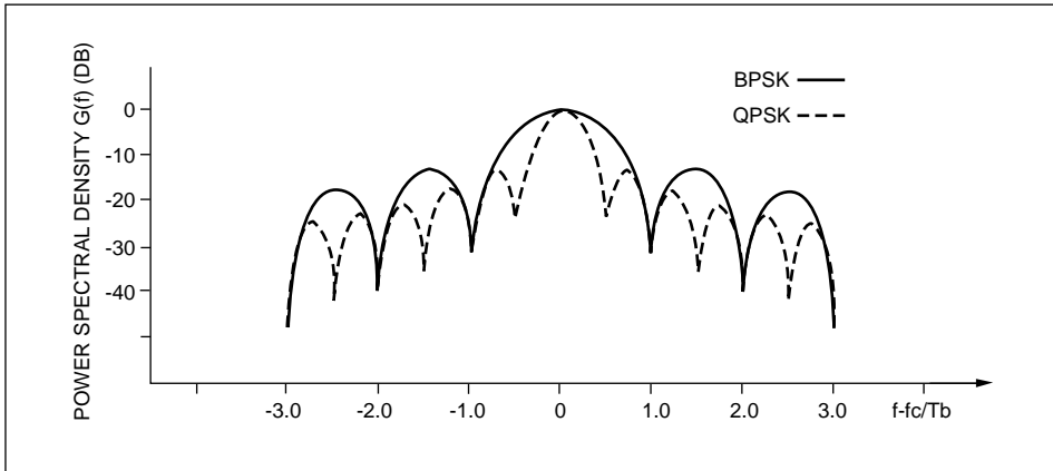
Figure 1. BPSK and QPSK spectra.
