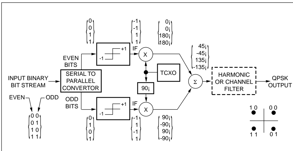
Figure 3. QPSK modulator.
