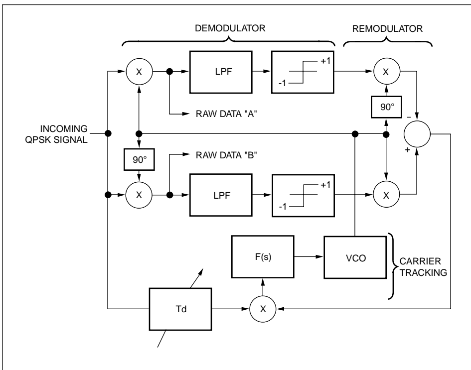
Figure 9. QPSK remodulator loop.
