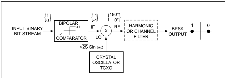
Figure 2. BPSK modulator.
