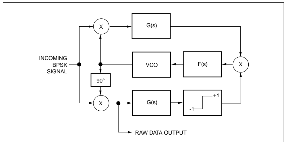
Figure 6. Hard-limited or polarity loop.
