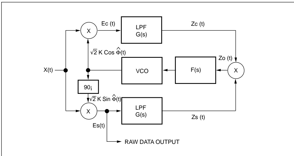
Figure 5. Conventional Costas loop.
